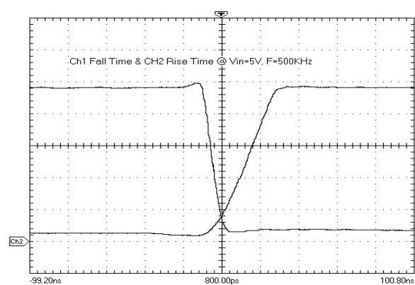
VCC= 5.0V, C1 = 15pF Channel 1 Fall Time Channel 2 Rise Time
