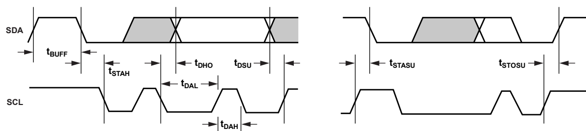
Figure 2. Serial Port Read/Write Timing
