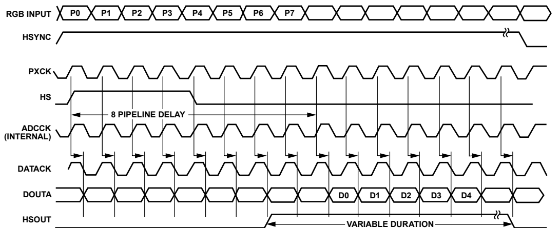
Figure 16. Single-Port Mode
