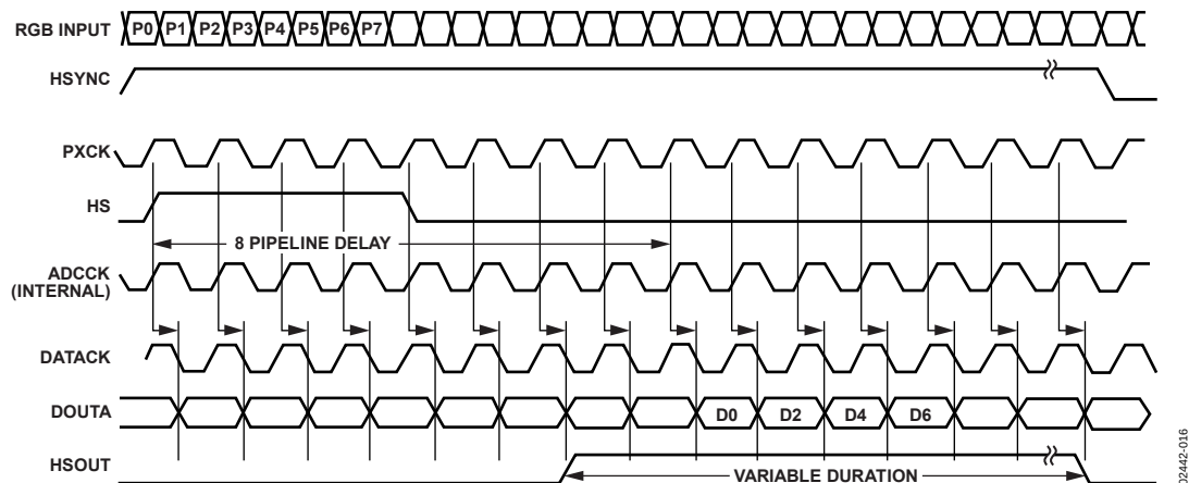
Figure 17. Single-Port Mode, Two Pixels/Clock (Even Pixels)
