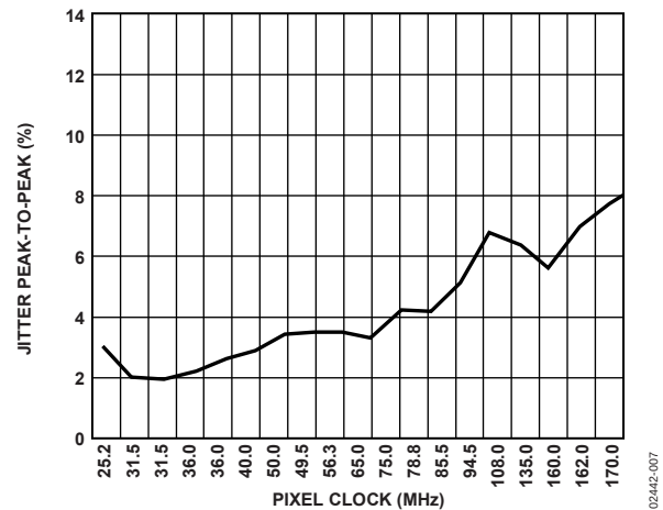
Figure 8. Pixel Clock Jitter vs. Frequency
