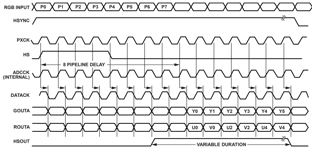
Figure 25. 4:2:2 Output Mode
