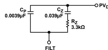
Figure 9. PLL Loop Filter Detail
