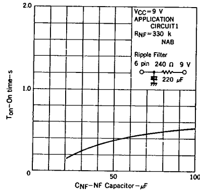
ON TIME vs. NF CAPACITOR
