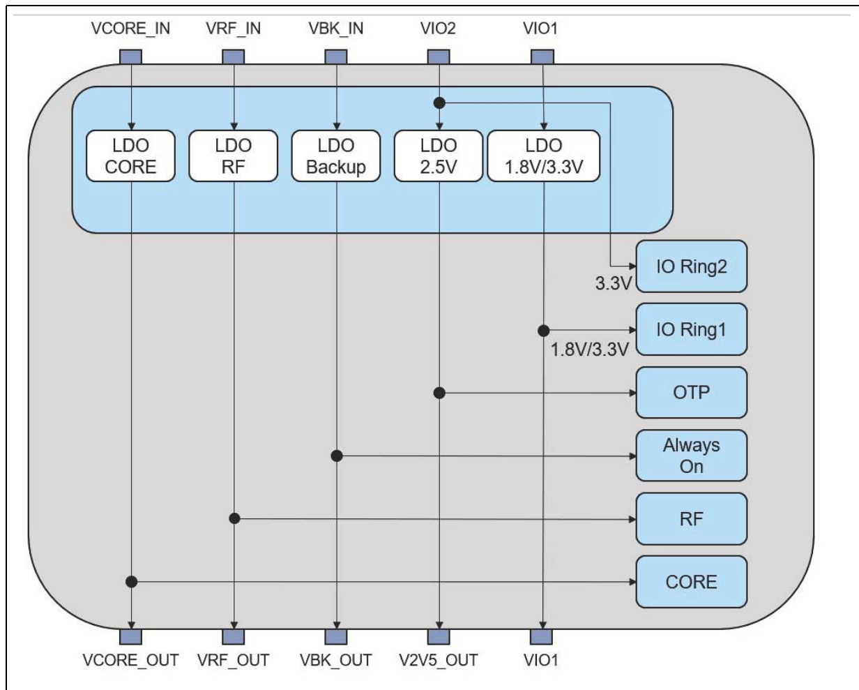
Figure 4. LDO on-chip regulators dependencies
