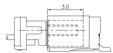
MATED CONDITION
