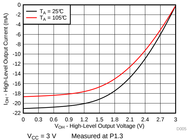
Figure 5-7. Typical High-Level Output Current vs High-Level Output Voltage
