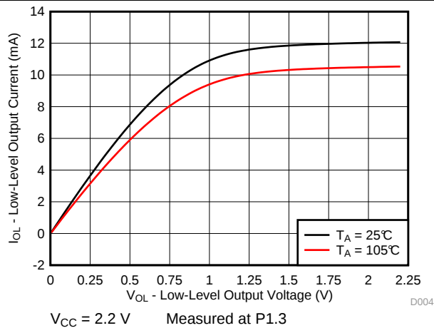
Figure 5-4. Typical Low-Level Output Current vs Low-Level Output Voltage
