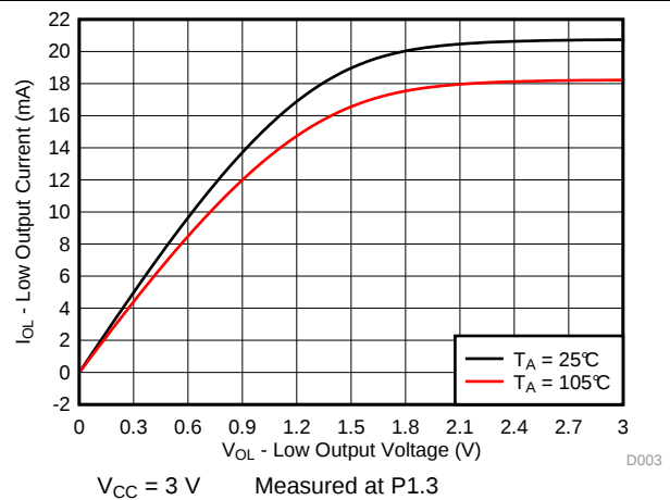
Figure 5-5. Typical Low-Level Output Current vs Low-Level Output Voltage
