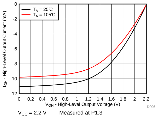
Figure 5-6. Typical High-Level Output Current vs High-Level Output Voltage
