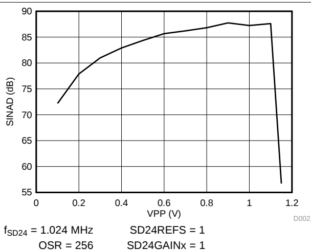
Figure 5-9. SINAD vs VPP
