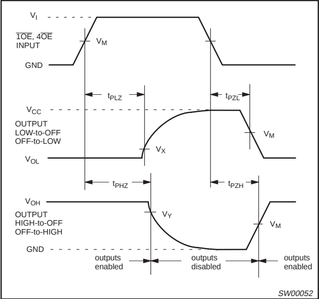
Waveform 3. 3-State enable and disable times for the input (1OE, 4OE)
