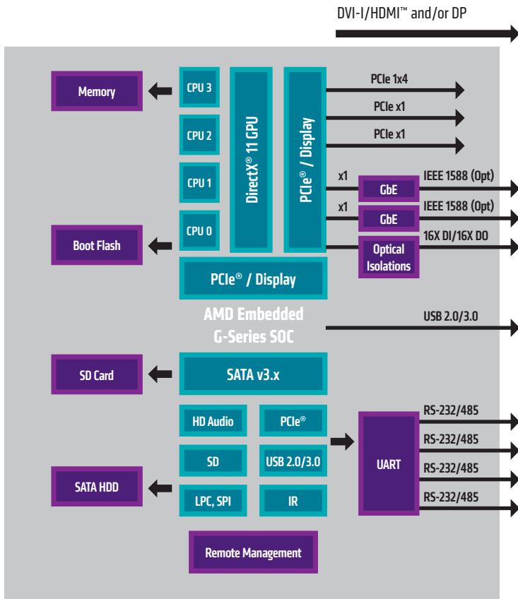
HIGH-PERFORMANCE BOX PC WITH AMD G-SERIES SOC
