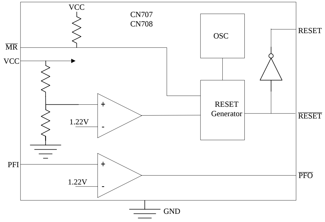
Figure 3 CN707/708 Block Diagram
