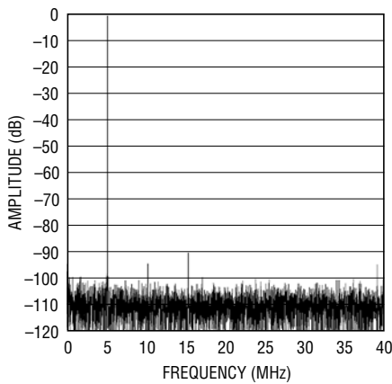
8192 Point FFT, f_{IN} = 5\text{MHz} , -1dB, 2V Range, 80Mps
