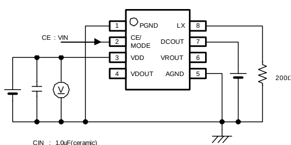
Circuit ⑥ Current Limit 1 (DC/DC)
