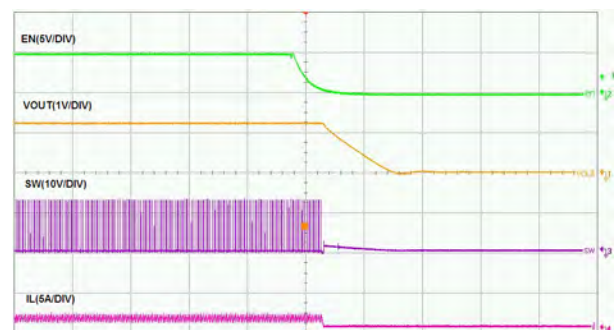
Time- 50µs/div Shutdown Through Enable ( I_{out} = 1A )
