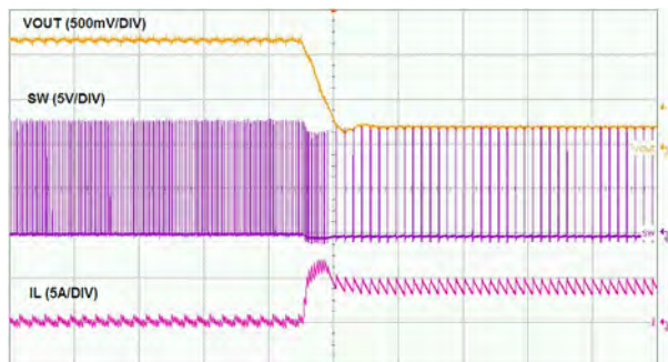
Time- 50µs/div Short Circuit Entry
