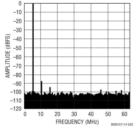
LTM9011-14: 8k Point FFT, f_{IN} = 5\text{MHz} , -1\text{dBFS} , 125Msps
