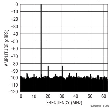
LTM9011-14: 8k Point FFT, f_{IN} = 140\text{MHz} , -1\text{dBFS} , 125Msps
