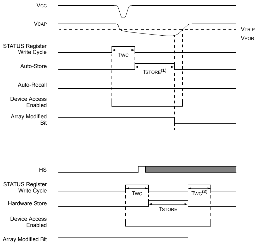
FIGURE 2-13: STORE DURING STATUS REGISTER WRITE CYCLE SCENARIOS (WITH AM = 1)
