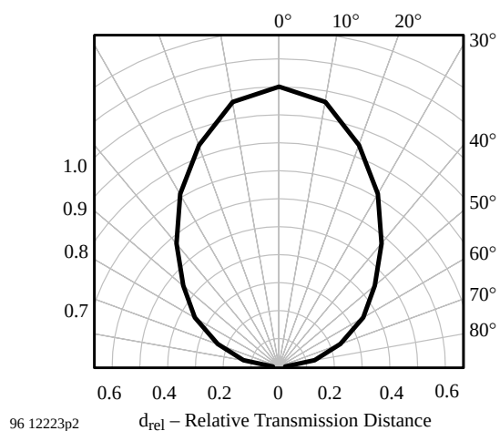
Figure 13. Directivity
