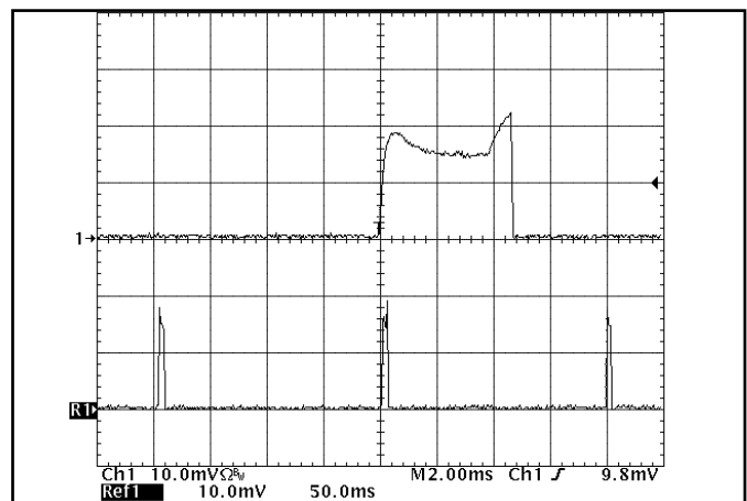
Figure 18: Load current (50A/div) as a function of time when the converter attempts to turn on into a 1\ \text{m}\Omega short circuit. Top trace (2ms/div) is an expansion of the on-time portion of the bottom trace.
