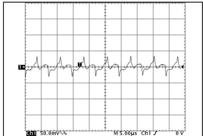
Figure 16: Output voltage ripple at nominal input voltage and rated load current (50 mV/div). Load capacitance: 1\ \mu\text{F} ceramic capacitor and 15\ \mu\text{F} tantalum capacitor. Bandwidth: 500 MHz. See Figure 13.
