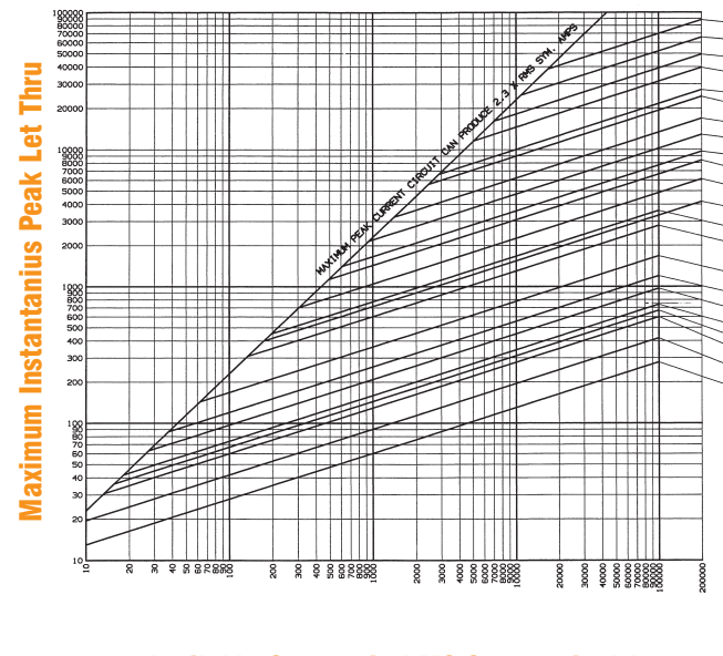
Peak Let Thru Data
