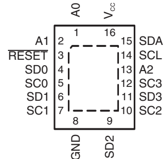
RGY PACKAGE (TOP VIEW)
