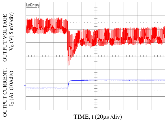
Transient Response to Dynamic Load Change from 50% to 100% at 12Vin, Cout-3x47uF+6x330uF, CTune-47nF, RTune-180ohms. Vo=0.6V
