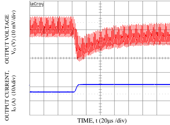
Transient Response to Dynamic Load Change from 50% to 100% at 12Vin, Cout-1x47uF+3x330uF, CTune-10nF & RTune-220ohms. Vo=1.2V
