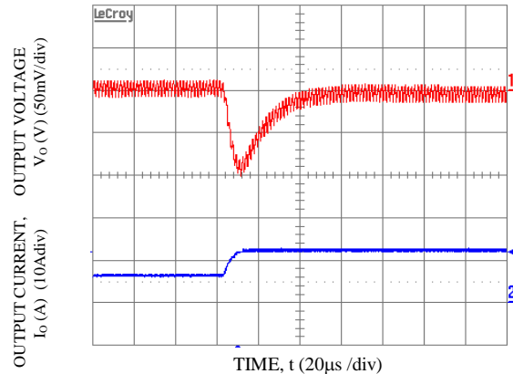
Transient Response to Dynamic Load Change from 50% to 100% at 12Vin, Cout-5x47uF, CTune-1500pF & RTune-330ohms. Vo=5.0V
