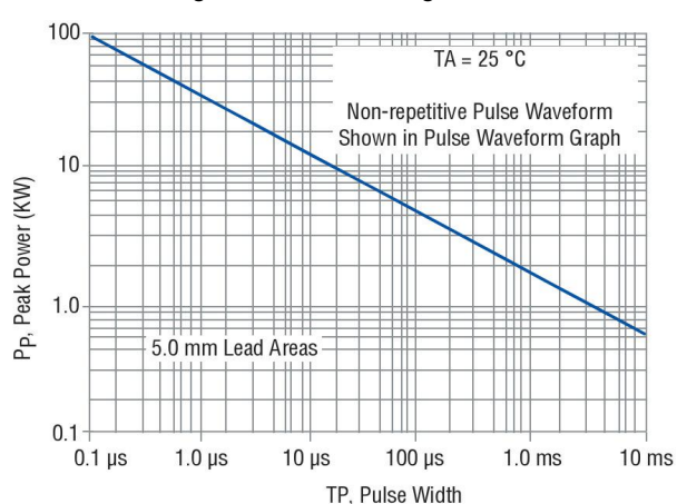
Figure 6- Pulse Rating Curve
