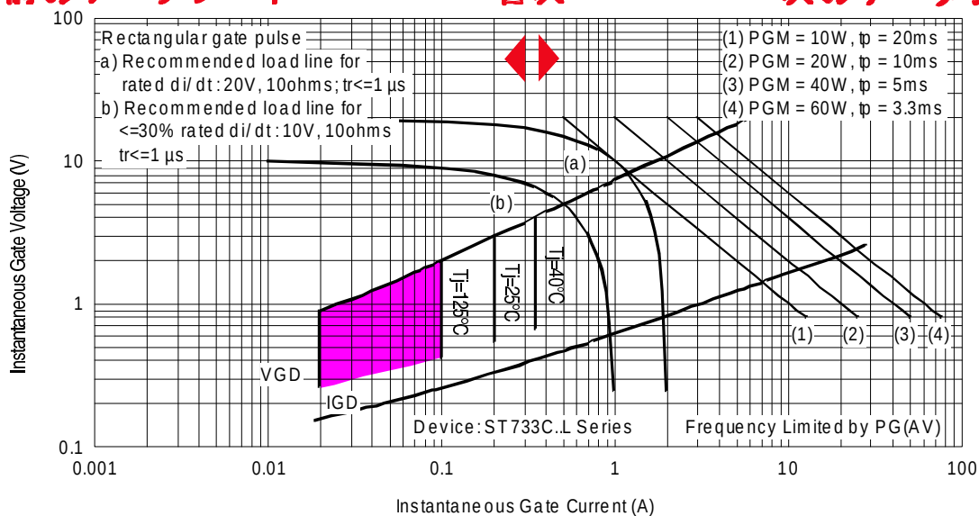
Fig. 17 - Gate Characteristics
