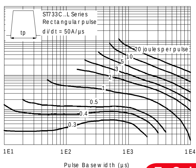
Fig. 16 - Maximum On-state Energy Power Loss Characteristics
