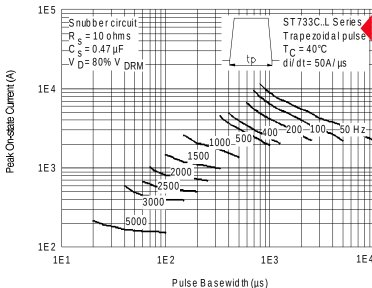
Fig. 14 - Frequency Characteristics
