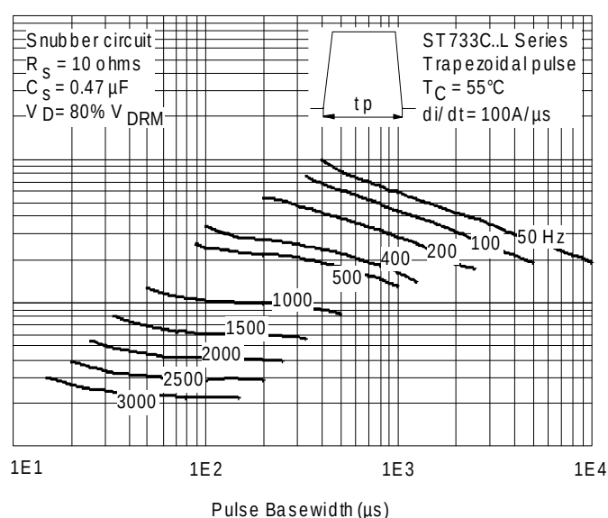
Fig. 15 - Frequency Characteristics
