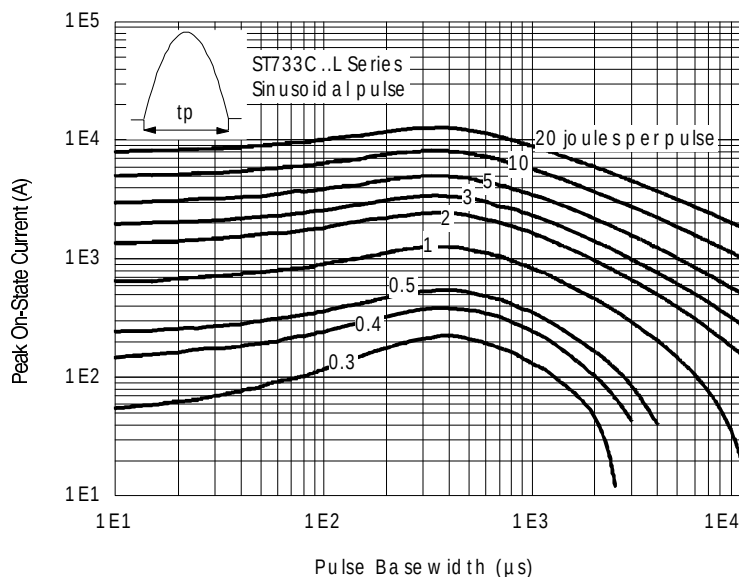
Fig. 16 - Maximum On-state Energy Power Loss Characteristics
