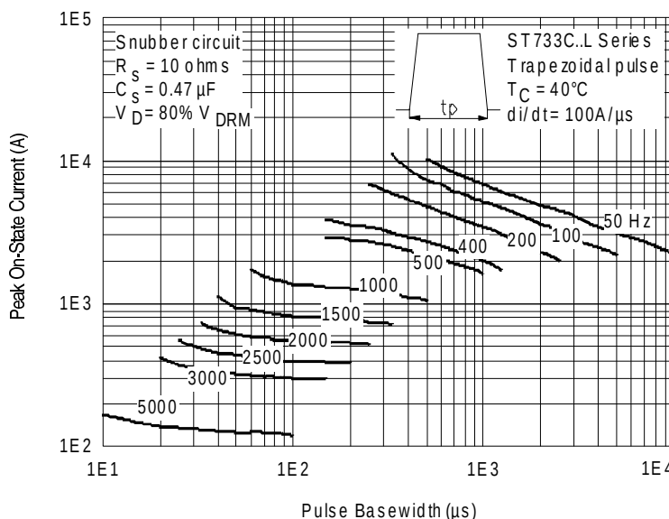
Fig. 15 - Frequency Characteristics
