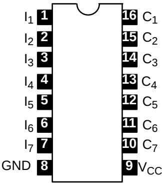
Pin Connection Diagram
