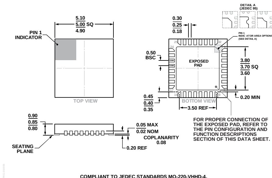
COMPLIANT TO JEDEC STANDARDS MO-220-VHHD-4. Figure 18. 32-Lead Lead Frame Chip Scale Package [LFCSP] 5 mm × 5 mm Body and 0.85 mm Package Height (HCP-32-1) Dimensions shown in millimeters
