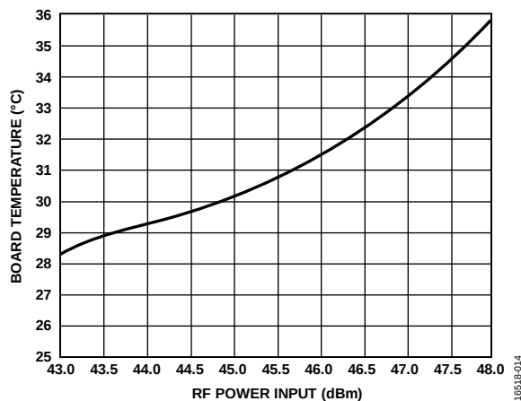
Figure 14. ADRF5160-EVALZ Evaluation Board Temperature Rise (Oven Temperature Set to 25°C)
