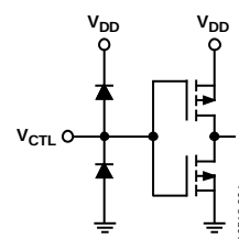
Figure 4. Control Input (V CTL ) Interface Schematic
