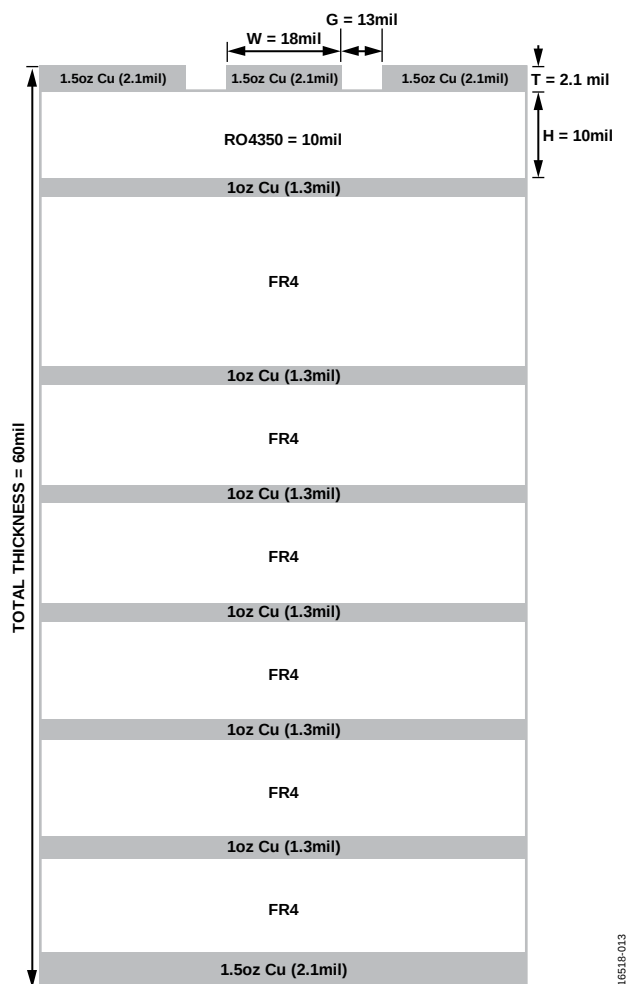
Figure 13. ADRF5160-EVALZ Evaluation Board Cross Sectional View
