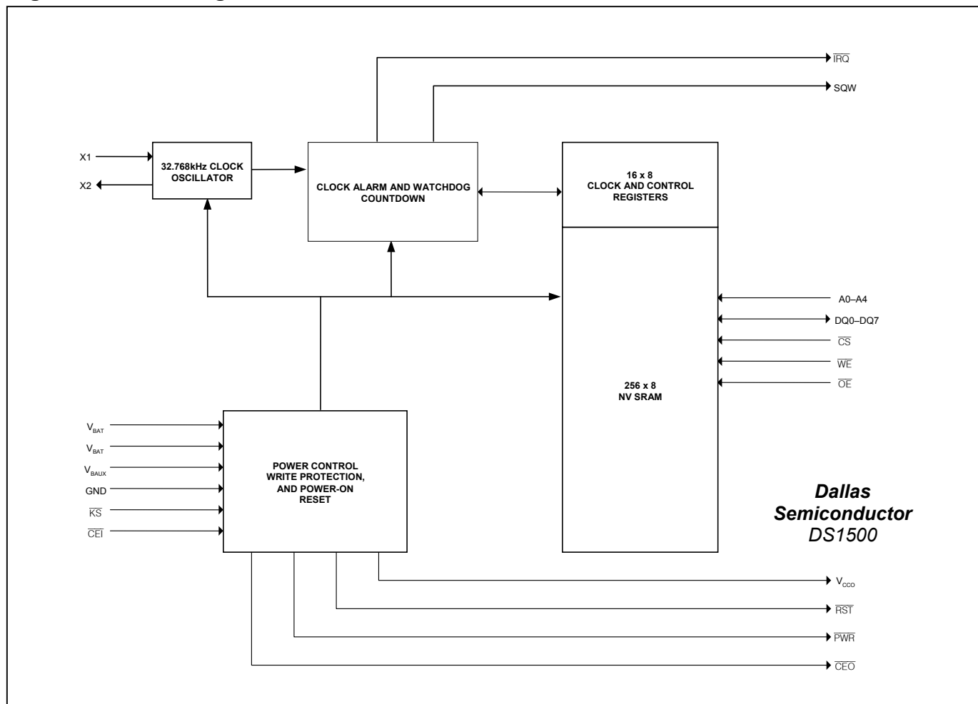
Figure 7. Block Diagram
