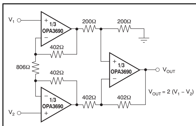
Figure 41. Instrumentation Amplifier
