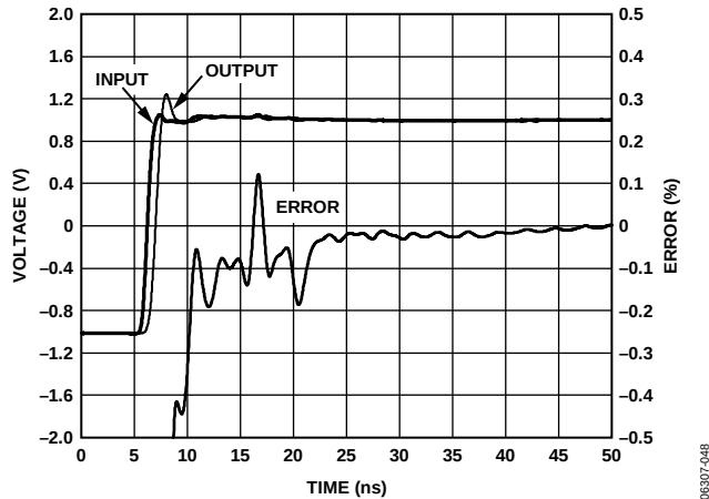
Figure 22. Settling Time
