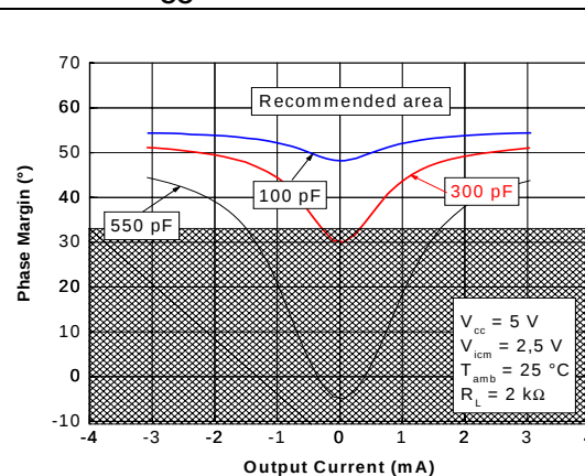
Figure 22. Phase margin vs. output current, at V_{CC}=5V and T=25^{\circ}C
