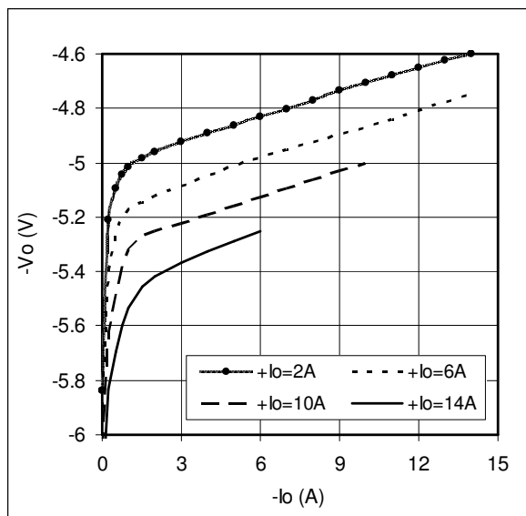
Figure 14 – DVFL2805D
