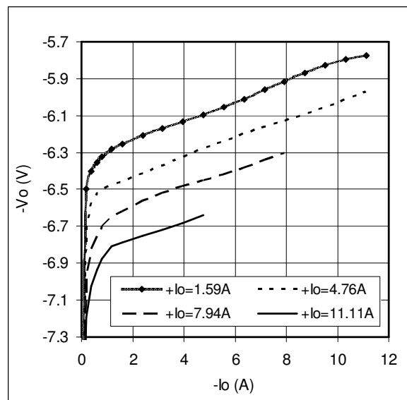
Figure 15 – DVFL286R3D
