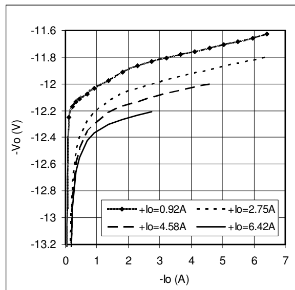
Figure 17 – DVFL2812D
