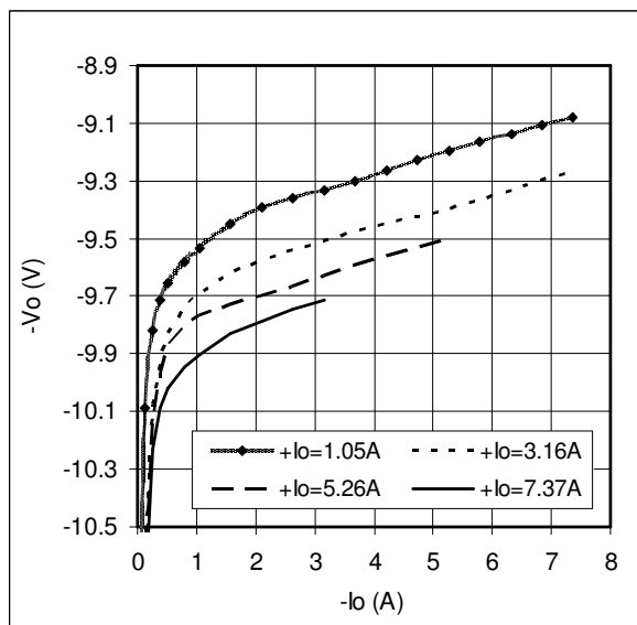
Figure 16 – DVFL289R5D
