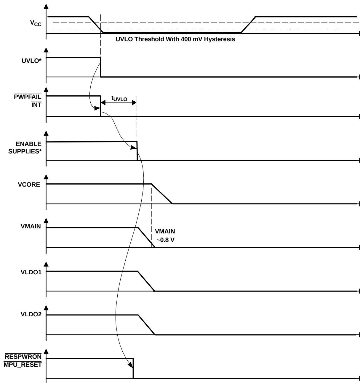
Figure 34. State 2 to State 4 Transition
