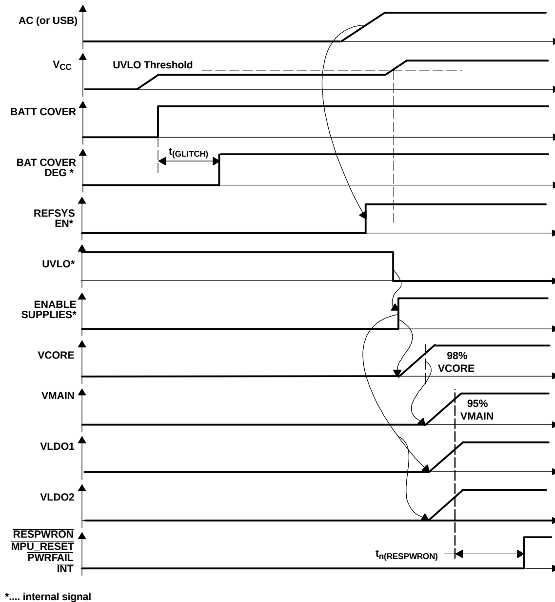
Figure 33. State 1 to State 4 to State 2 Transition (Power up Behavior When Charge Voltage is Applied)
