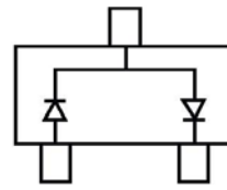
BAS40-04 MARKING: 44
