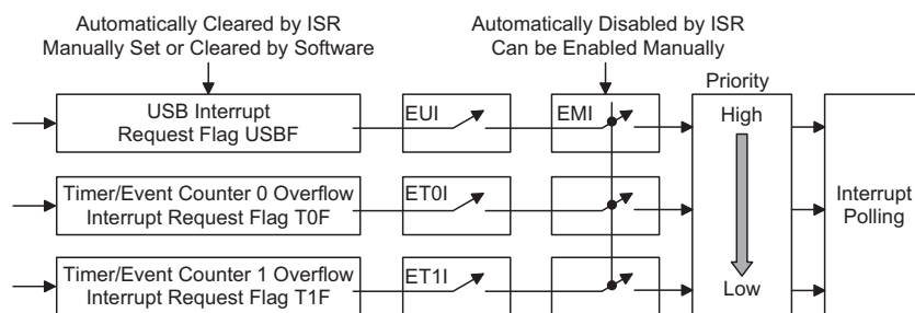
Interrupt Structure
