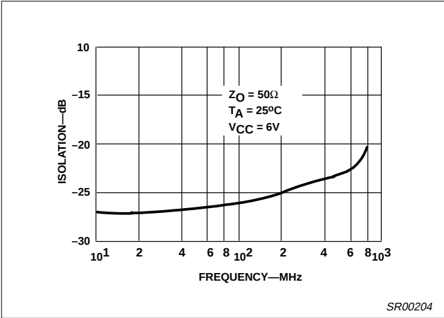
Figure 14. Isolation vs Frequency (S 12 )
