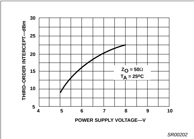
Figure 10. Third-Order Intercept vs Supply Voltage
