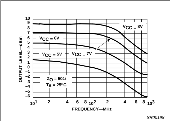
Figure 8. 1dB Gain Compression vs Frequency
