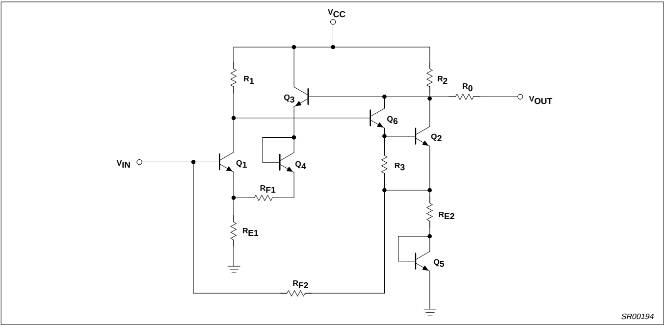
Figure 2. Equivalent Schematic
