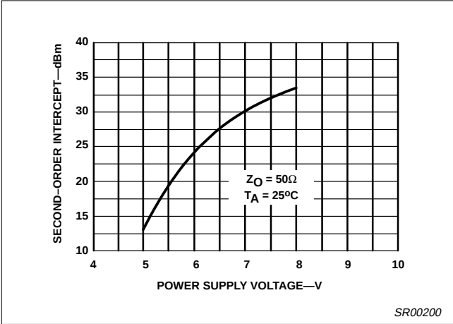
Figure 9. Second-Order Output Intercept vs Supply Voltage
