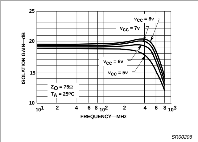
Figure 15. Insertion Gain vs Frequency (S 21 )
