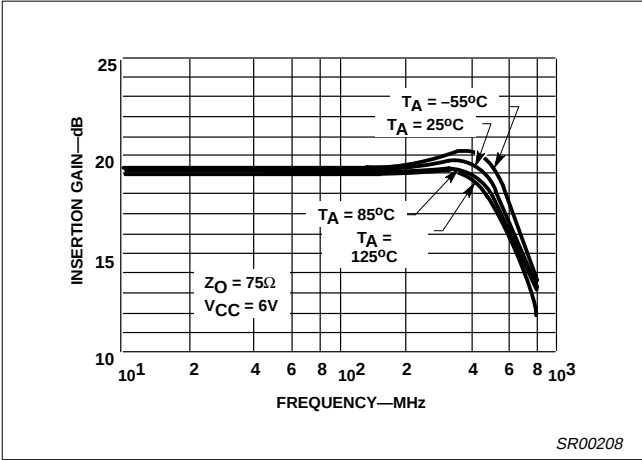
Figure 16. Insertion Gain vs Frequency (S 21 )
