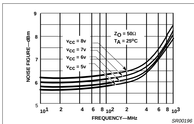
Figure 4. Noise Figure vs Frequency
