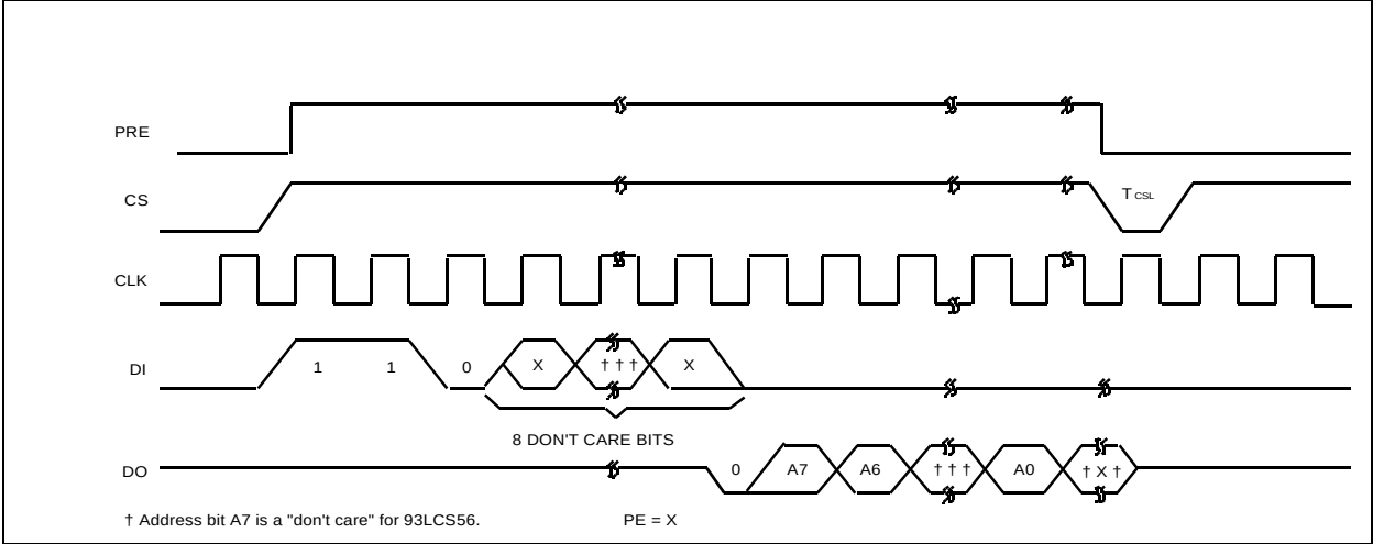
FIGURE 2-9: PRREAD TIMING
