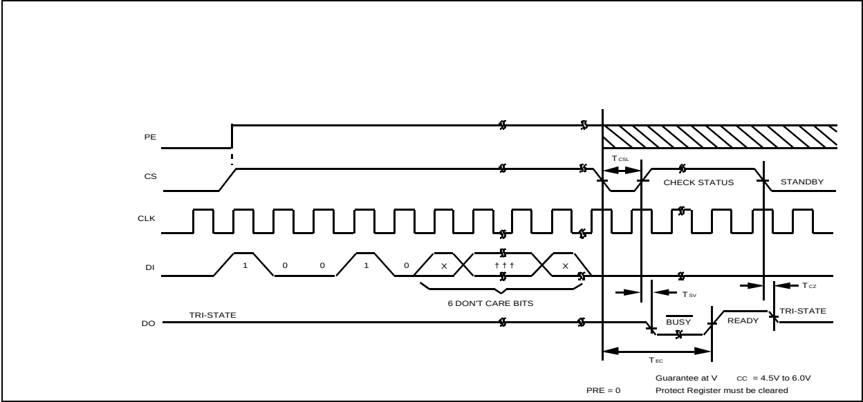
FIGURE 2-9: PRREAD TIMING
