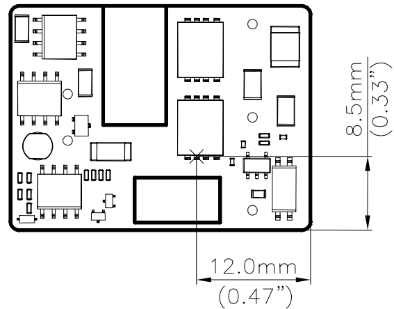
Figure 20: Hot spot temperature measured point
