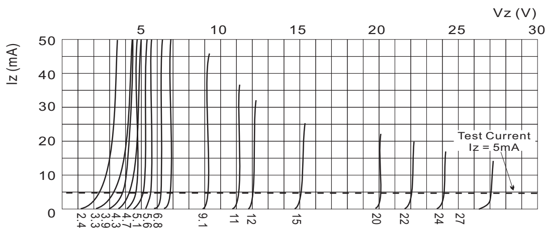
Fig. 2 Z-Current vs. Z-Voltage
