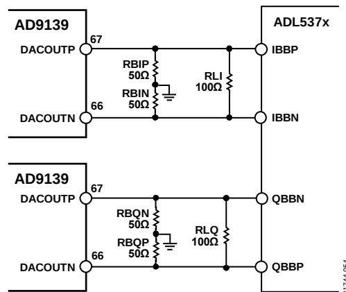
Figure 49. Typical Interface Circuitry Between the AD9139 and the ADL537x Family of Modulators
