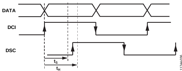
Figure 31. LVDS Data Port Setup and Hold Times
