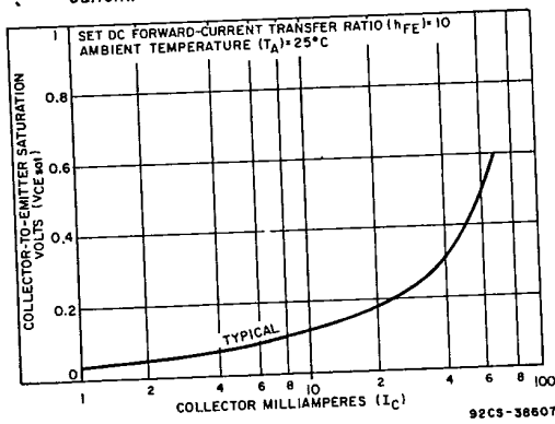
Fig. 4 - Collector-to-emitter saturation voltage as a function of collector current at T_A = 25^\circ\text{C} .
