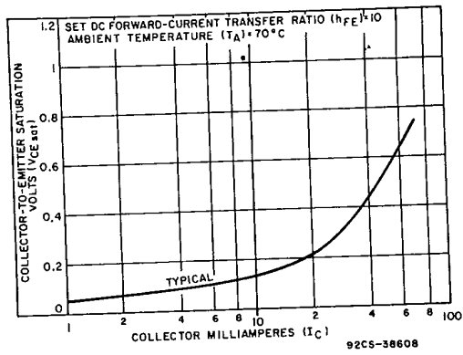
Fig. 5 - Collector-to-emitter saturation voltage as a function of collector current at T_A = 70^\circ\text{C} .
