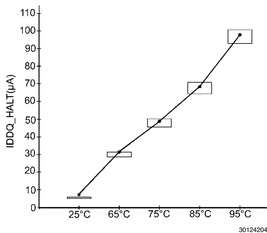
FIGURE 3. Halt Current vs. Temperature at 1.98V
