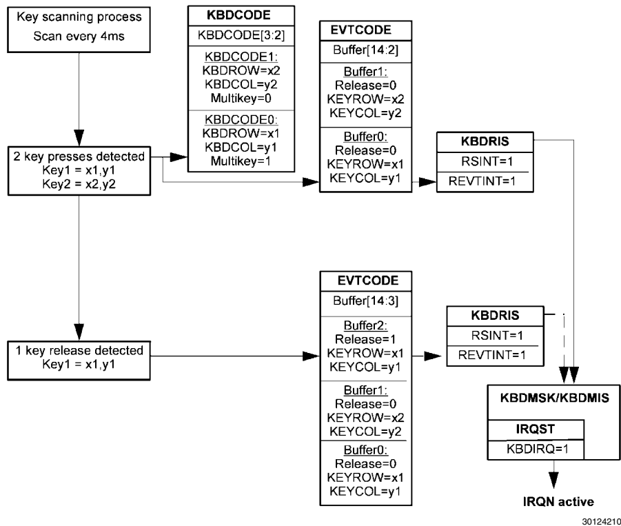
FIGURE 9. Example Keyscan Operation for 2 Key Press Events and 1 Key Release Event
