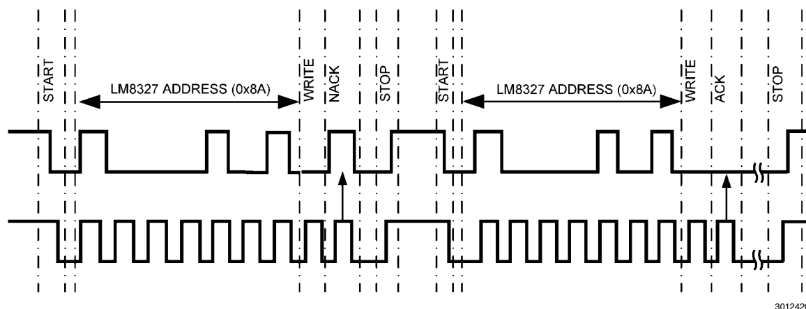
FIGURE 5. Host Starts Communication While LM8327 is in Sleep Mode
