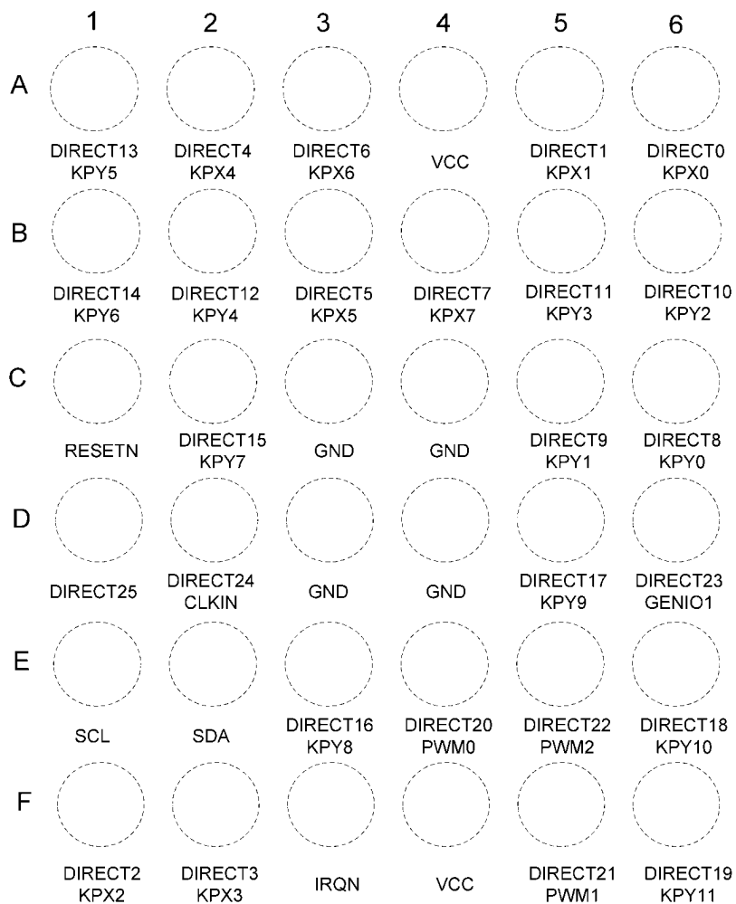
FIGURE 1. LM8327 Pinout - Top View
