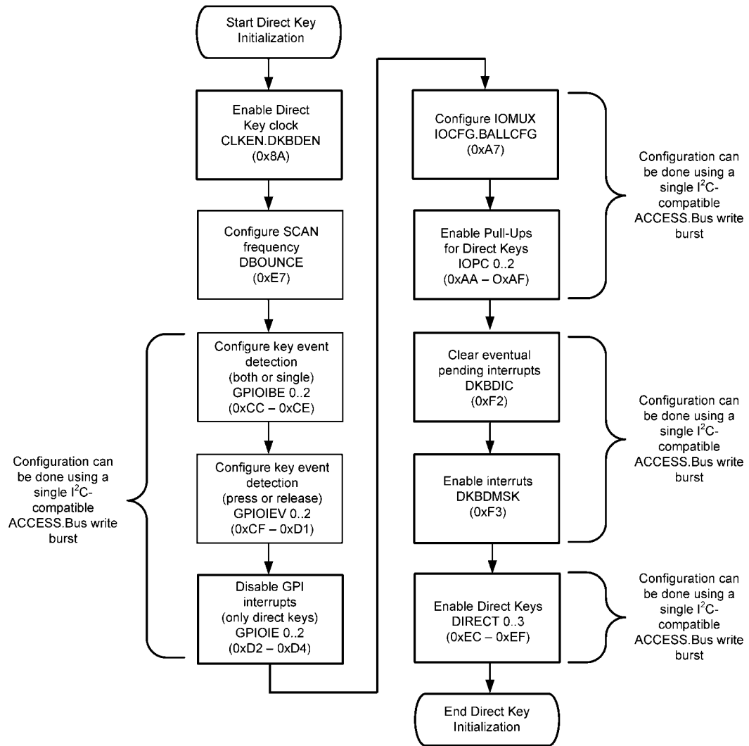
FIGURE 10. Direct Key Initialization
