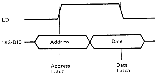
Fig. 4 – ADDRESS/DATA FORMAT
