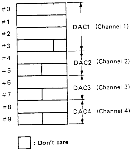
Fig. 5 – INTERNAL DATA REGISTER ADDRESS MAP
