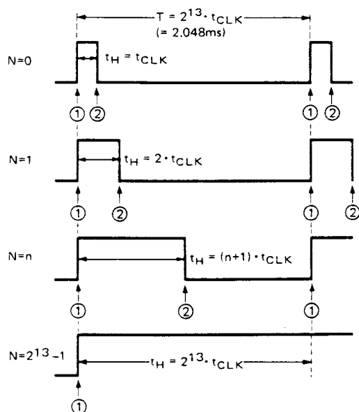
Fig. 8 – DAC1 OUTPUT WAVEFORM
