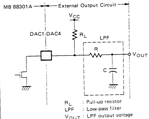
Fig. 11 — OUTPUT CIRCUIT CONFIGURATION (EXAMPLE)
