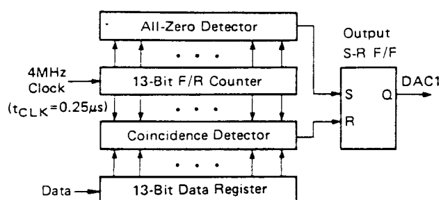
Fig. 7 – 13-BIT PULSE WIDTH MODULATOR CONFIGURATION
