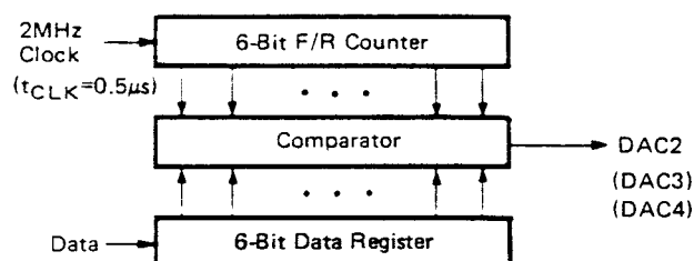
Fig. 9 – 6-BIT PULSE WIDTH MODULATOR CONFIGURATION
