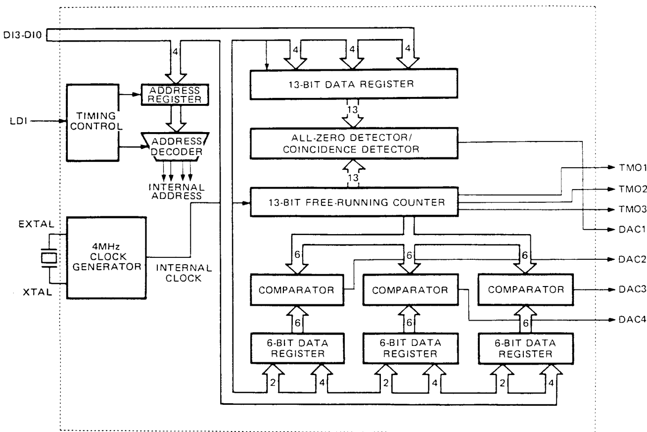
Fig. 2 – BLOCK DIAGRAM
