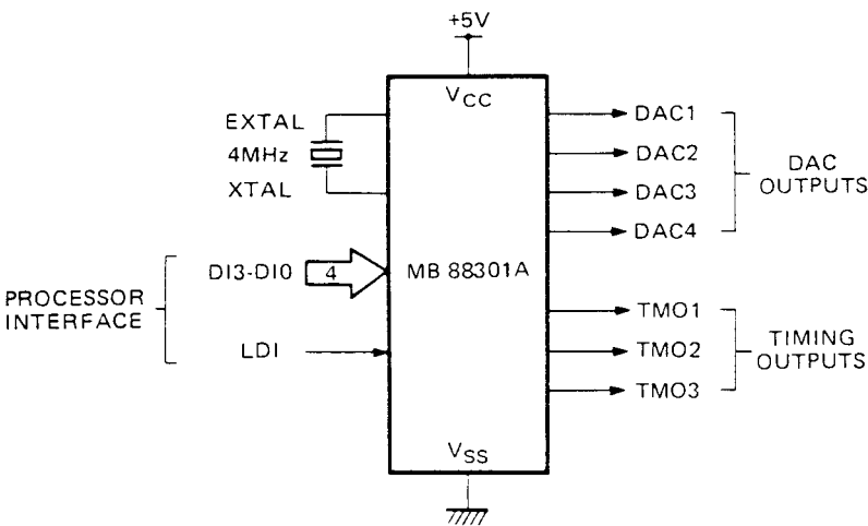
Fig. 1 – LOGIC SYMBOL
