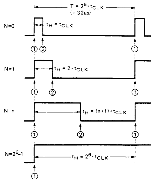
Fig. 10 – DAC2/DAC3/DAC4 OUTPUT WAVEFORM
