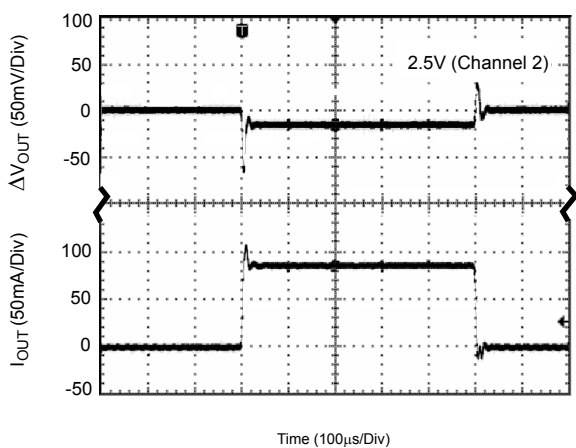
Figure 38. Load Transient
