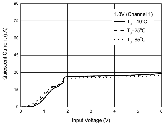
Figure 24. Quiescent Current vs. Input Voltage
