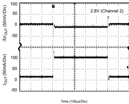
Figure 39. Load Transient
