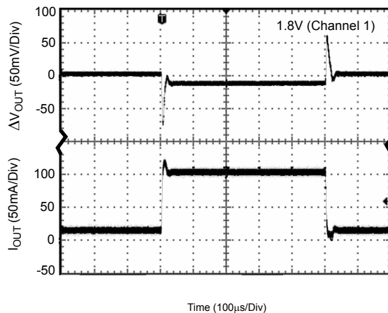
Figure 37. Load Transient
