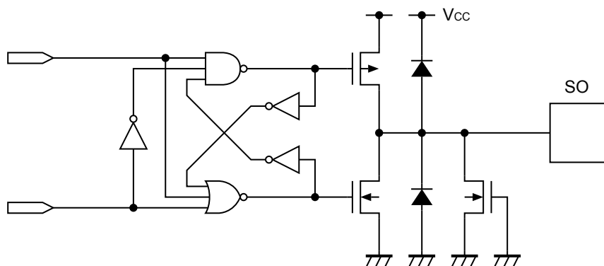
Figure 22 SO Pin
