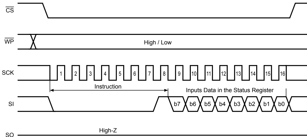
Figure 14 WRSR Operation
