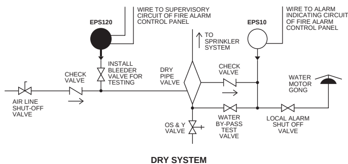
DRY SYSTEM
