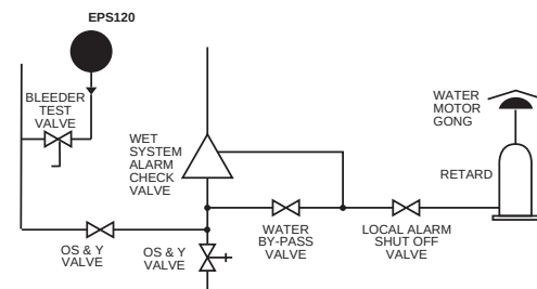
WET SYSTEM
