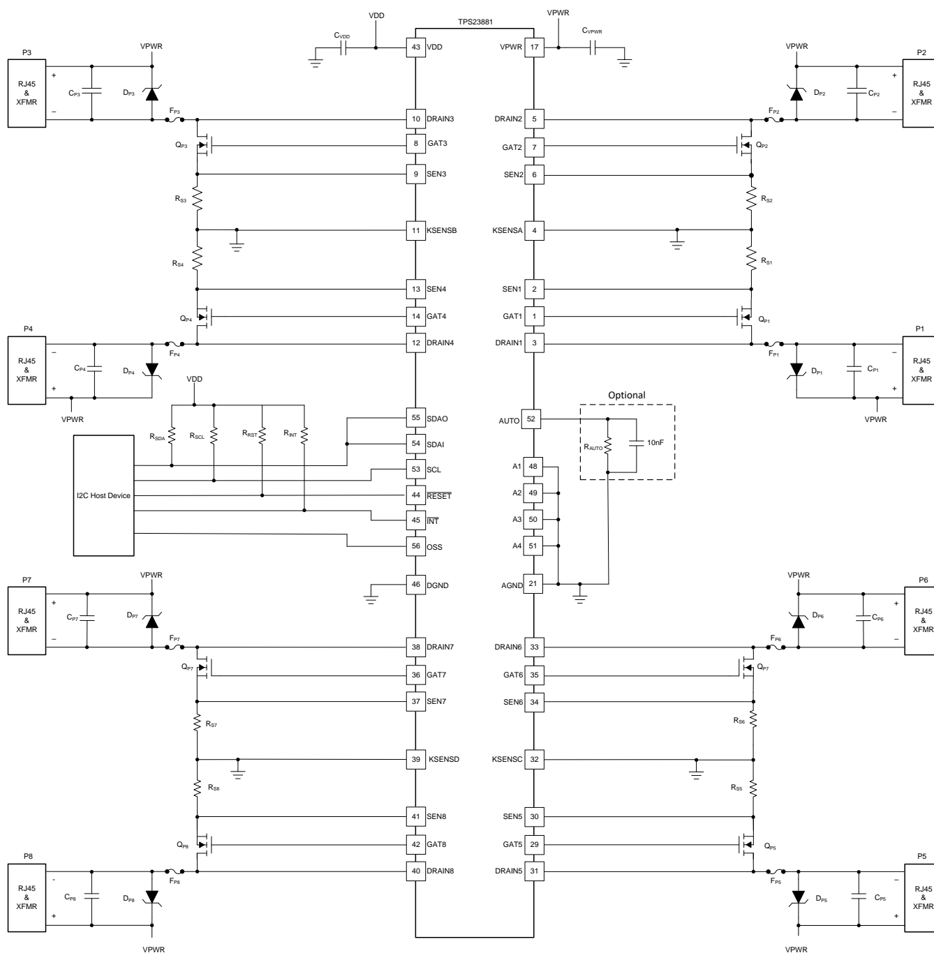
Figure 92. Eight 2-Pair Port Application
