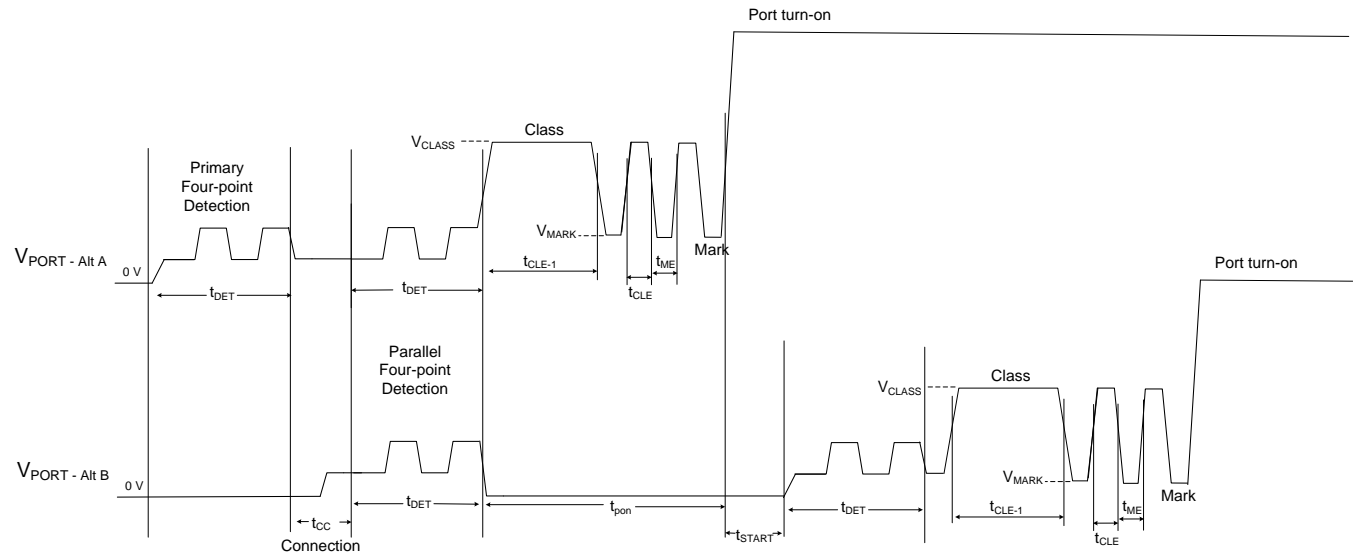
Figure 7. 4-Pair Dual Signature Detection, 3-Event Classification and Turn On
