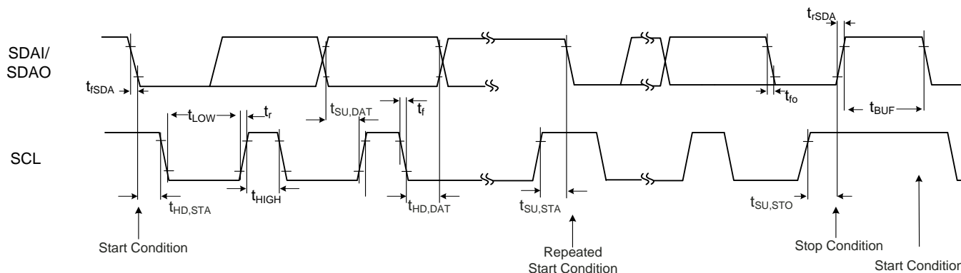
Figure 1. I²C Timings
