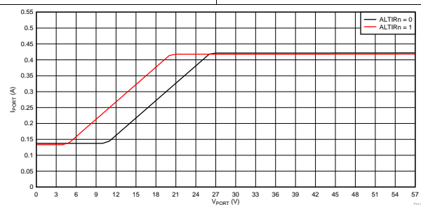
Figure 88. Inrush Foldback Curves, I_{PORT} vs V_{PORT}
