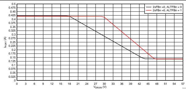
Figure 86. 1x Mode (2xFBn = 0) Foldback Curves, I_{PORT} vs V_{DRAIN}
