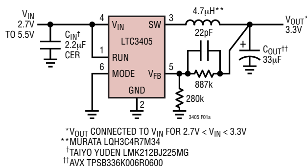
Figure 1a. High Efficiency Step-Down Converter
