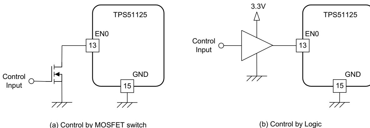
Figure 38. Control Example of EN0 Master Enable
