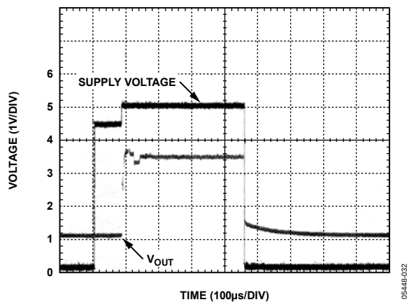
Figure 31. Power-On Response at 125°C
