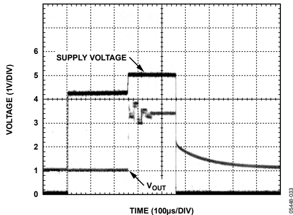
Figure 32. Power-On Response at -40°C
