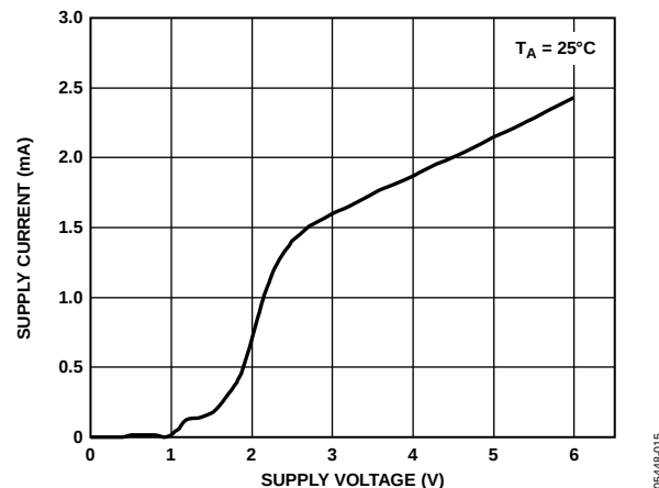
Figure 14. Supply Current ( I_{SV} ) vs. Supply Voltage
