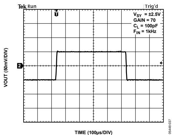
Figure 36. Small Signal Response at C_L = 100\text{ pF} and F_{IN} = 1\text{ kHz}
