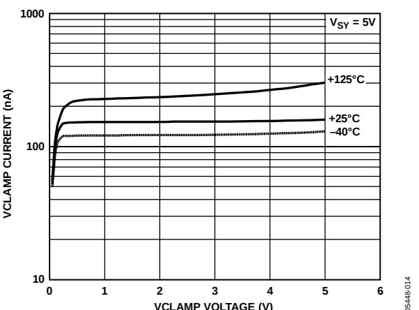
Figure 13. VCLAMP Current over Temperature at V_S = 5V vs. VCLAMP Voltage
