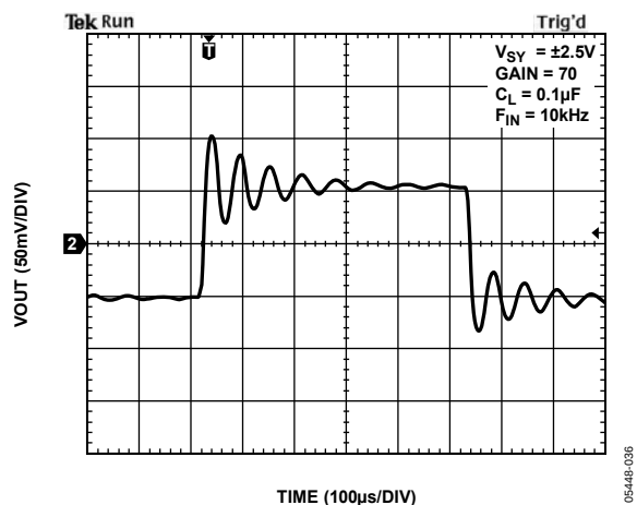
Figure 35. Small Signal Response at C_L = 0.1\text{ }\mu\text{F} and F_{IN} = 10\text{ kHz}
