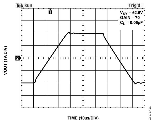
Figure 38. Large Signal Response at C_L = 0.05\text{ }\mu\text{F}
