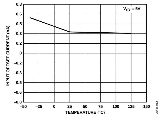
Figure 11. Input Offset Current vs. Temperature
