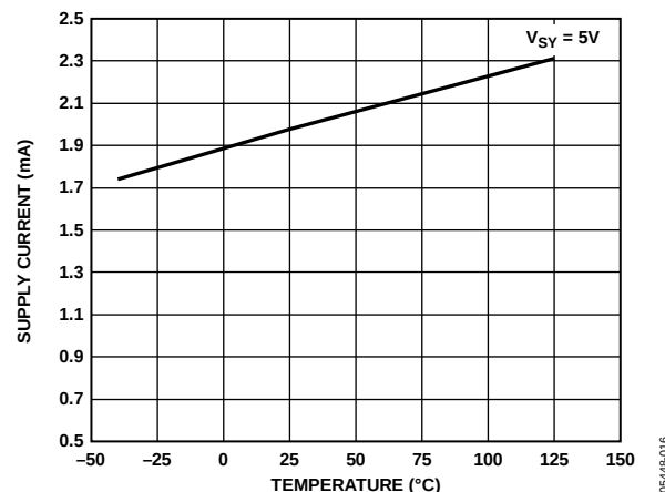
Figure 15. Supply Current ( I_{SV} ) vs. Temperature
