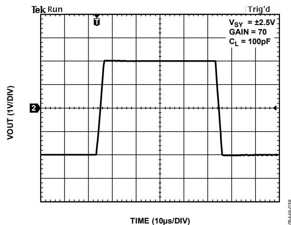
Figure 37. Large Signal Response at C_L = 100\text{ pF}
