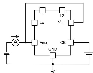
< Circuit No.③ >
