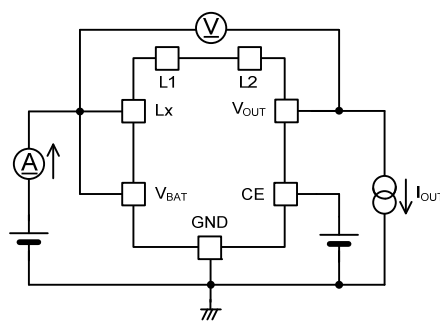
< Circuit No.④ >
