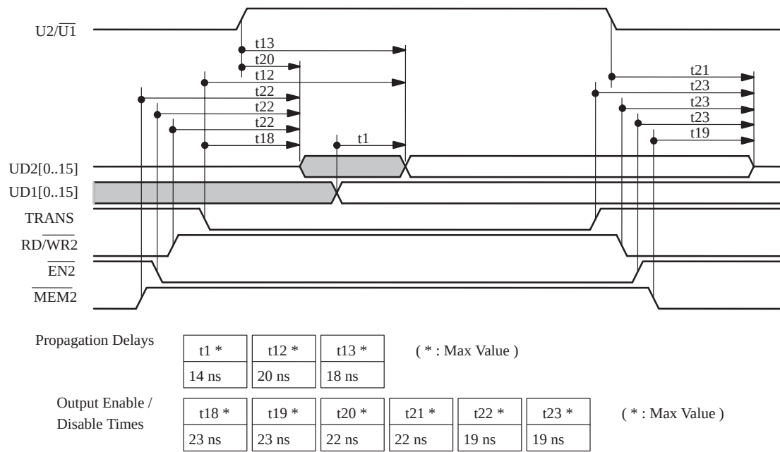
Figure 7. Transfer Read Timing Diagram
