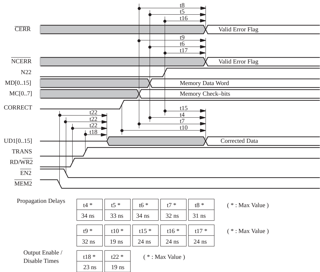
Figure 6.Memory Read Timing Diagram
