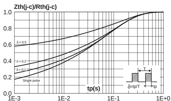
Fig. 6-1: Relative variation of thermal impedance junction to case versus pulse duration (per diode).
