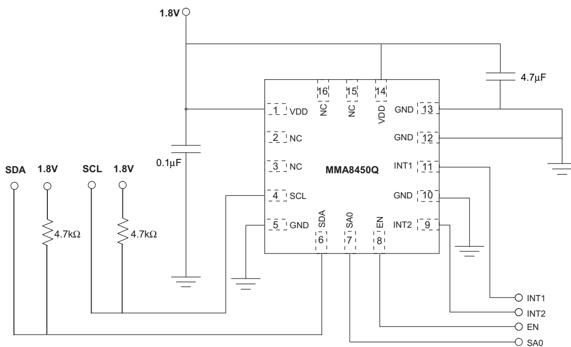
Figure 4. Application Diagram
